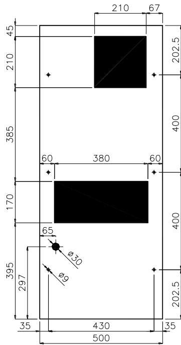
MONTAGE EXTERNE / EXTERNAL MOUNTED
